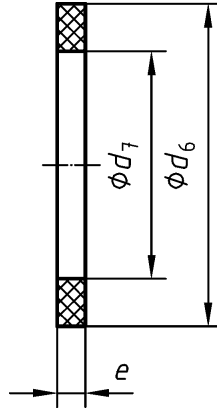
Figure 8 – Gasket
