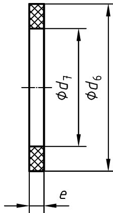
Figure 8 – Joint
